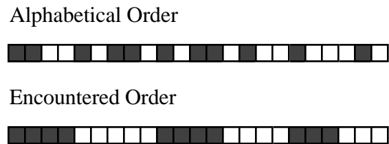
Figure 5: Non-empty entries in a sparse table, as influenced by selector code
