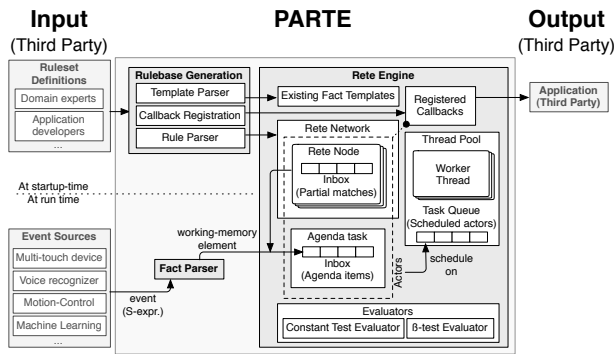
Figure 2. The architecture of PARTE
