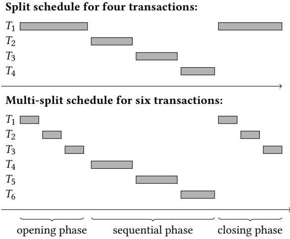
Figure 2: Abstract presentation of split and multi-split schedule. The drawing omits a possible trailing sequence of non-interleaved transactions (cf. Definition 8 and Definitions 18).
