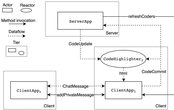
Figure 1: Communication/dataflow diagram of the CoCode application with two clients (one client fully drawn).
